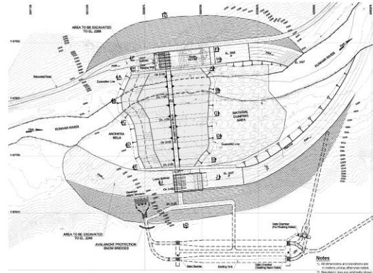
Layout Plan
