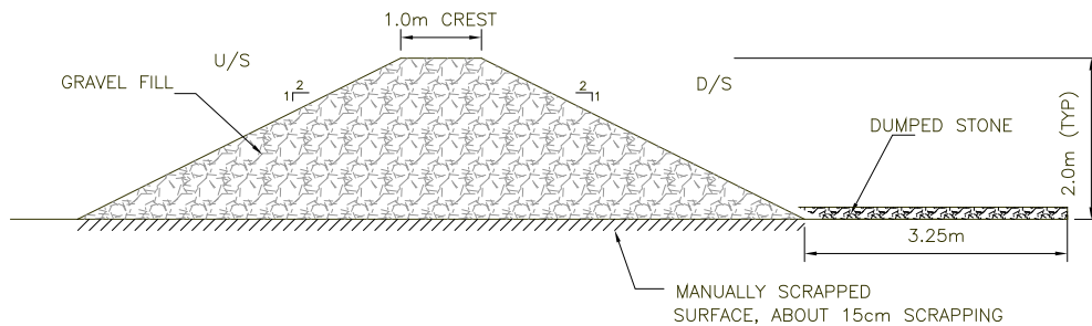
CHECK DAM
